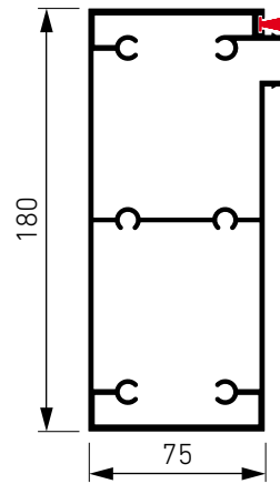
Beam P-180x85 mm ■ 050206
