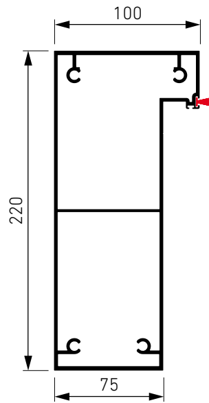
Beam P-220x100 mm ■ 023103
