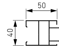
Clipp-on adapter 40x50 mm SOFT ■ 050218
